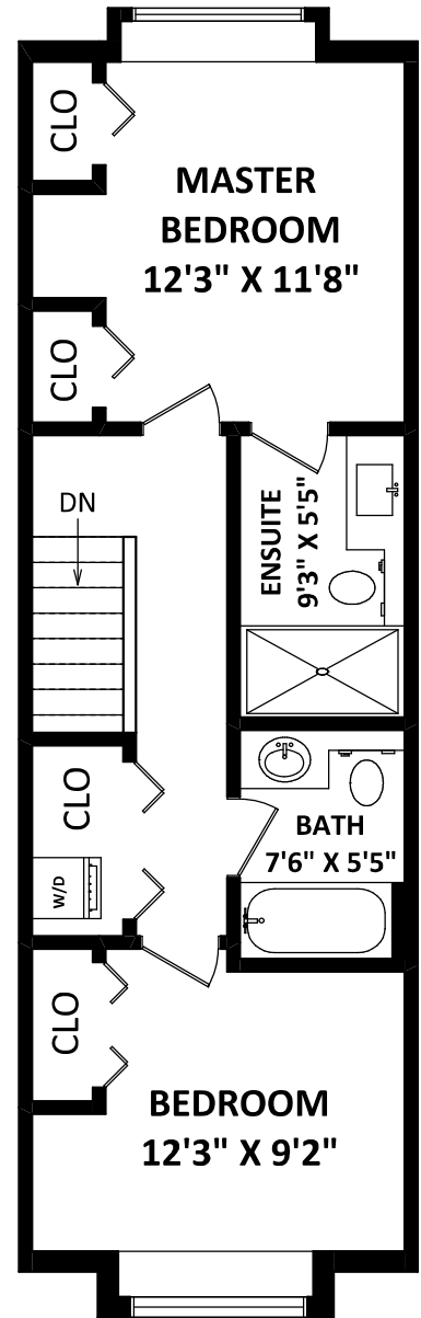
UPPER FLOOR: 540 SQ.FT.
