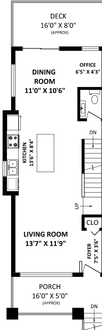
MAIN FLOOR: 671 SQ.FT.
